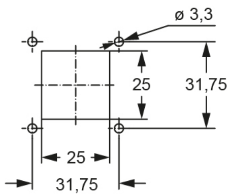
Catalogue drawings
