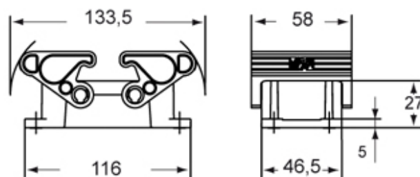
Catalogue drawings
