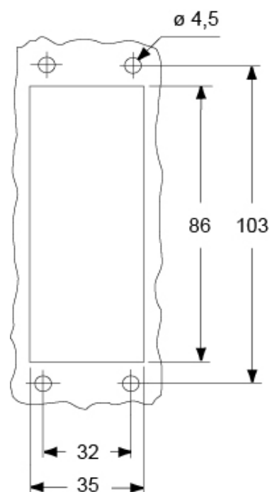
Catalogue drawings
