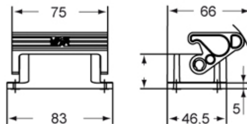
Catalogue drawings
