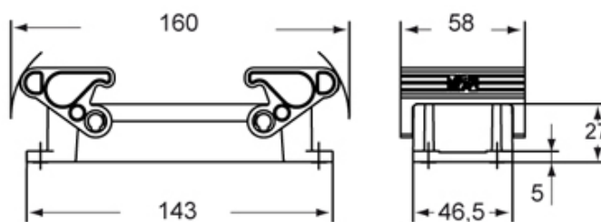
Catalogue drawings
